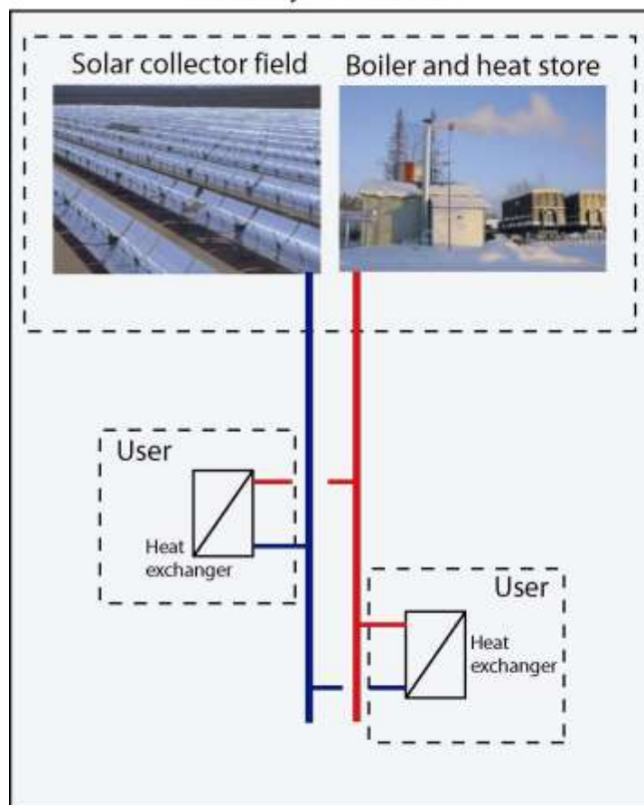
Central system solution
