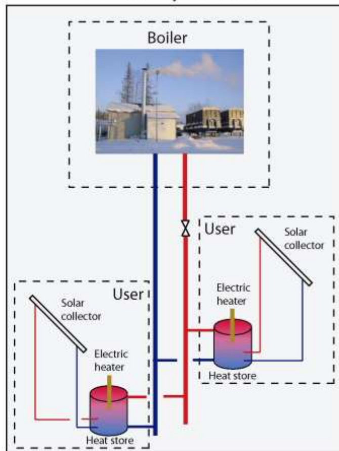
Distributed system solution
